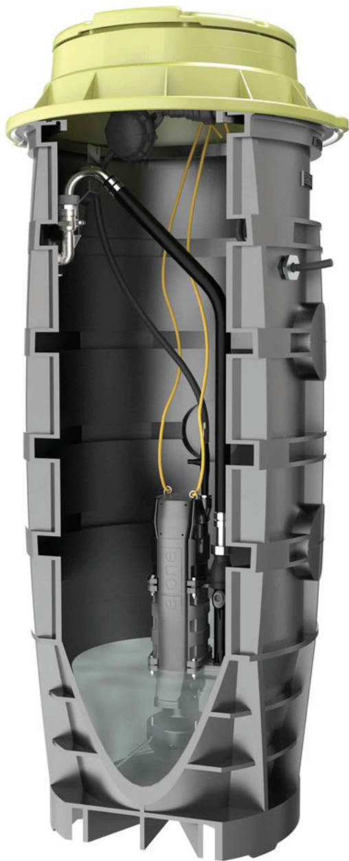
E/One Simplex 2010iP – single pump
